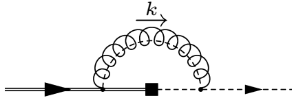
FIG. 3: Contribution of the additional SCET II mode proposed in Refs. [9].
